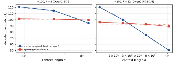
(b) End-to-end throughput vs n (batch 1).
